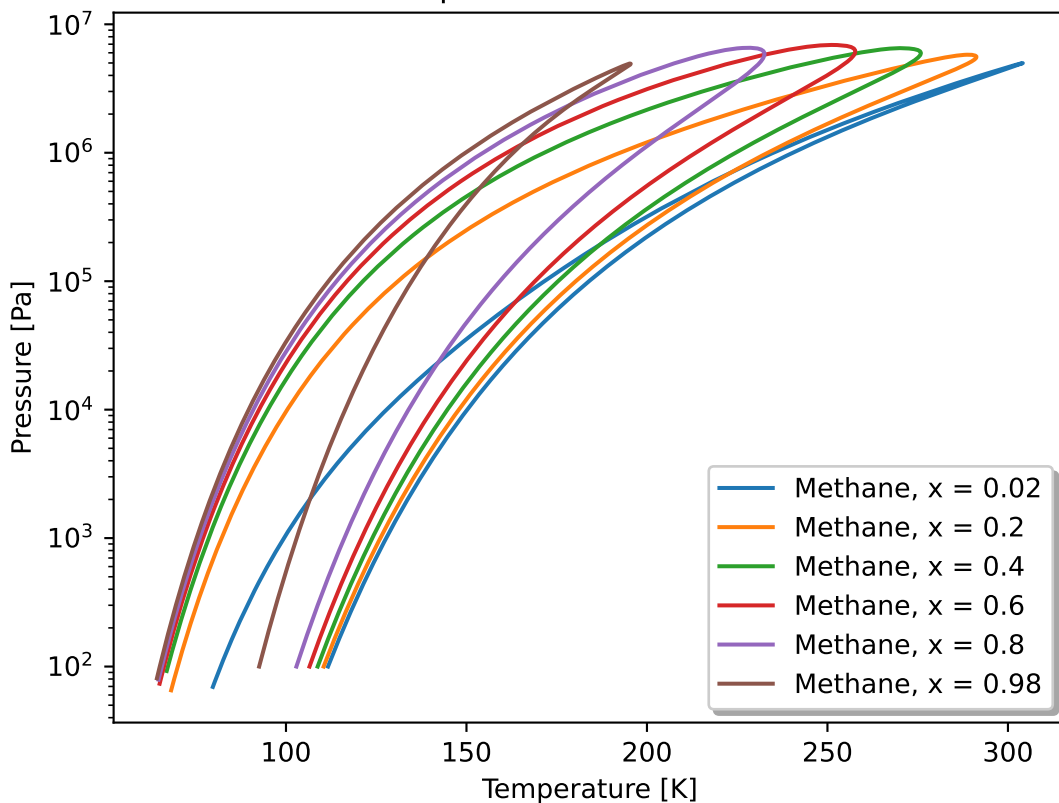
Phase Envelope for Methane/Ethane Mixtures
