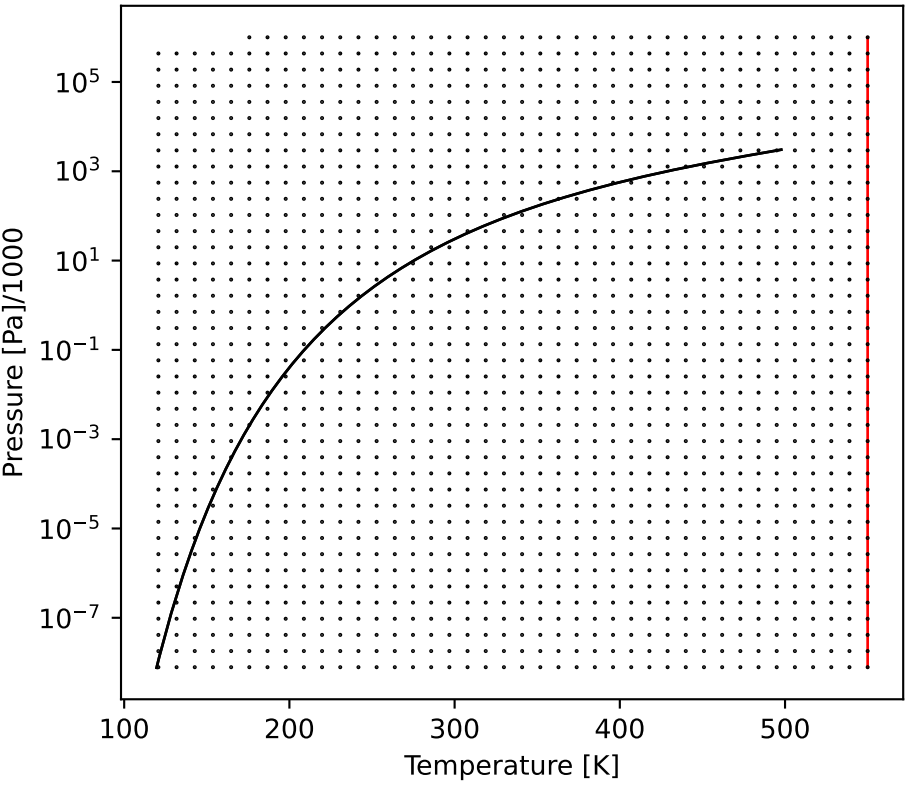
PSmolar
