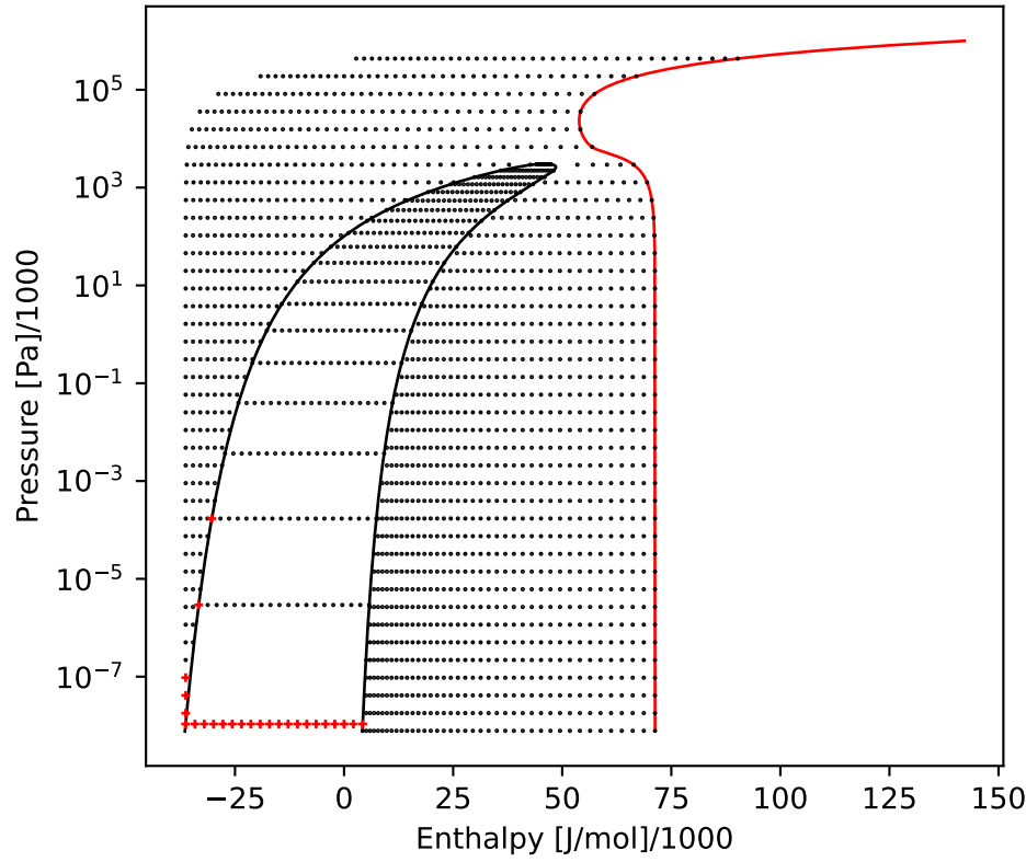
PUmolar
