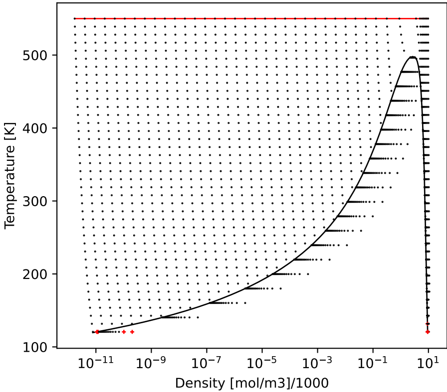
SmolarT
