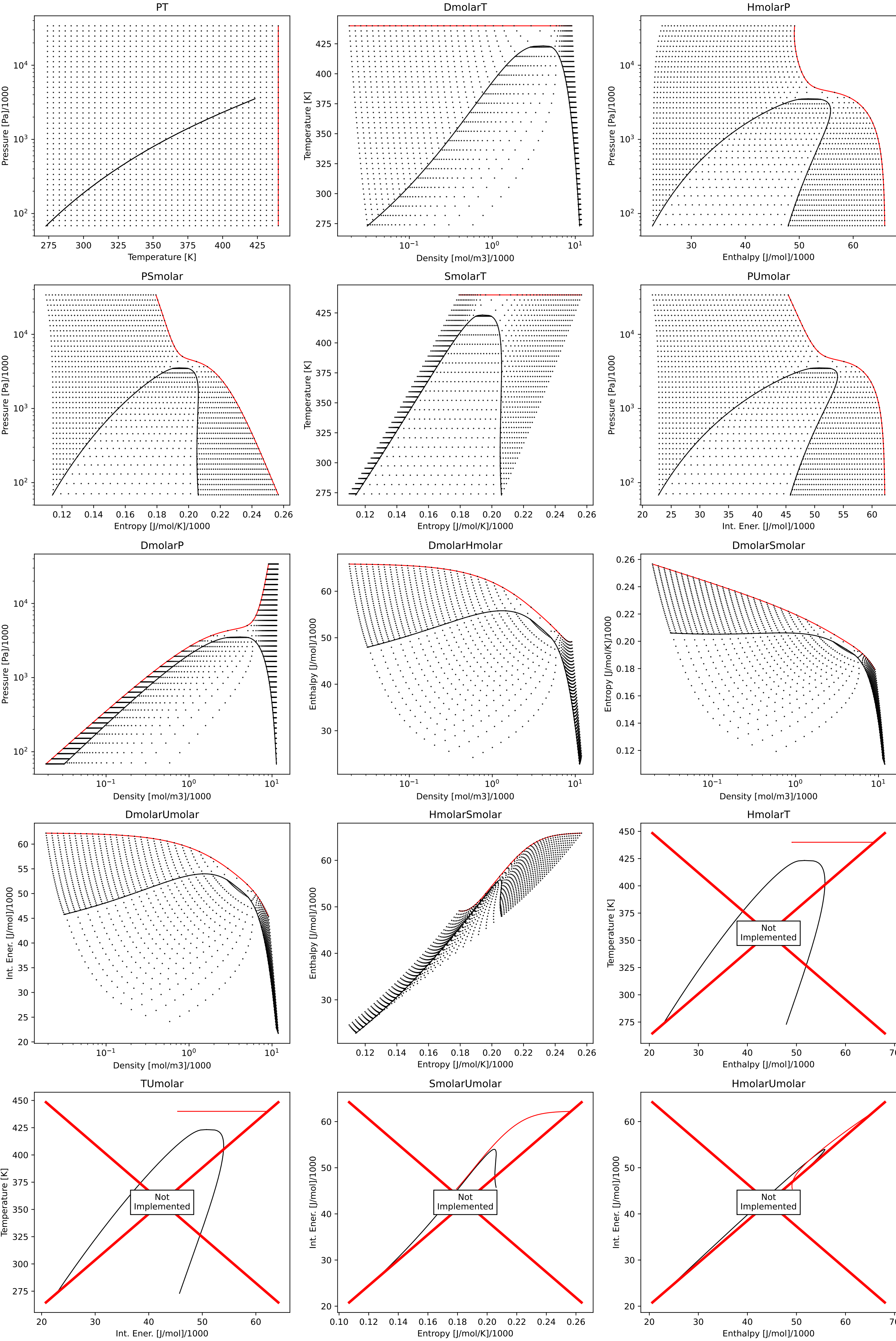
Consistency plots for R1234ze(Z)
