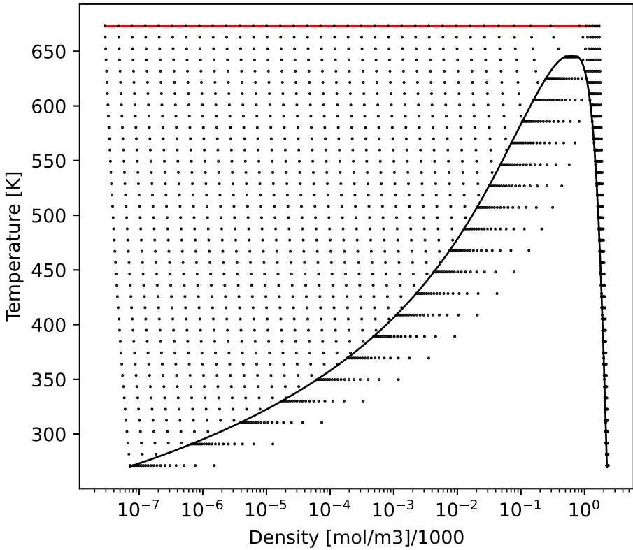
SmolarT
