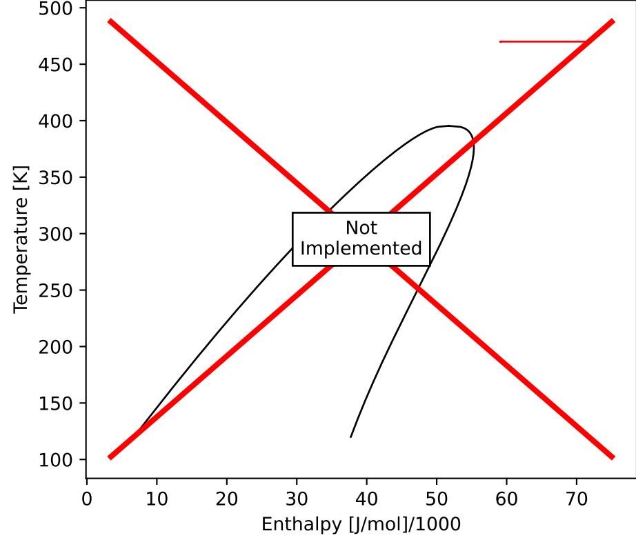
HmolarUmolar
