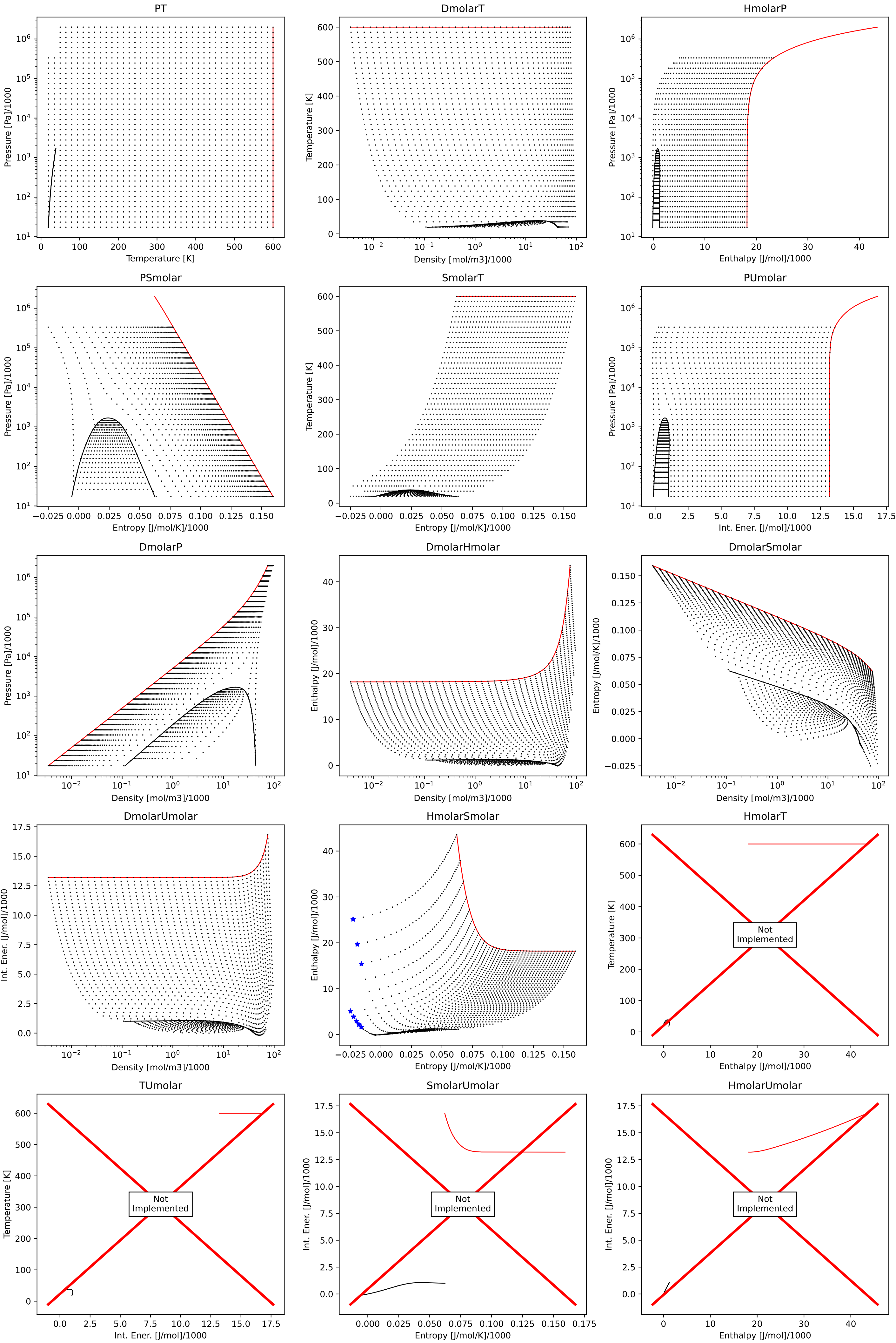
Consistency plots for OrthoDeuterium
