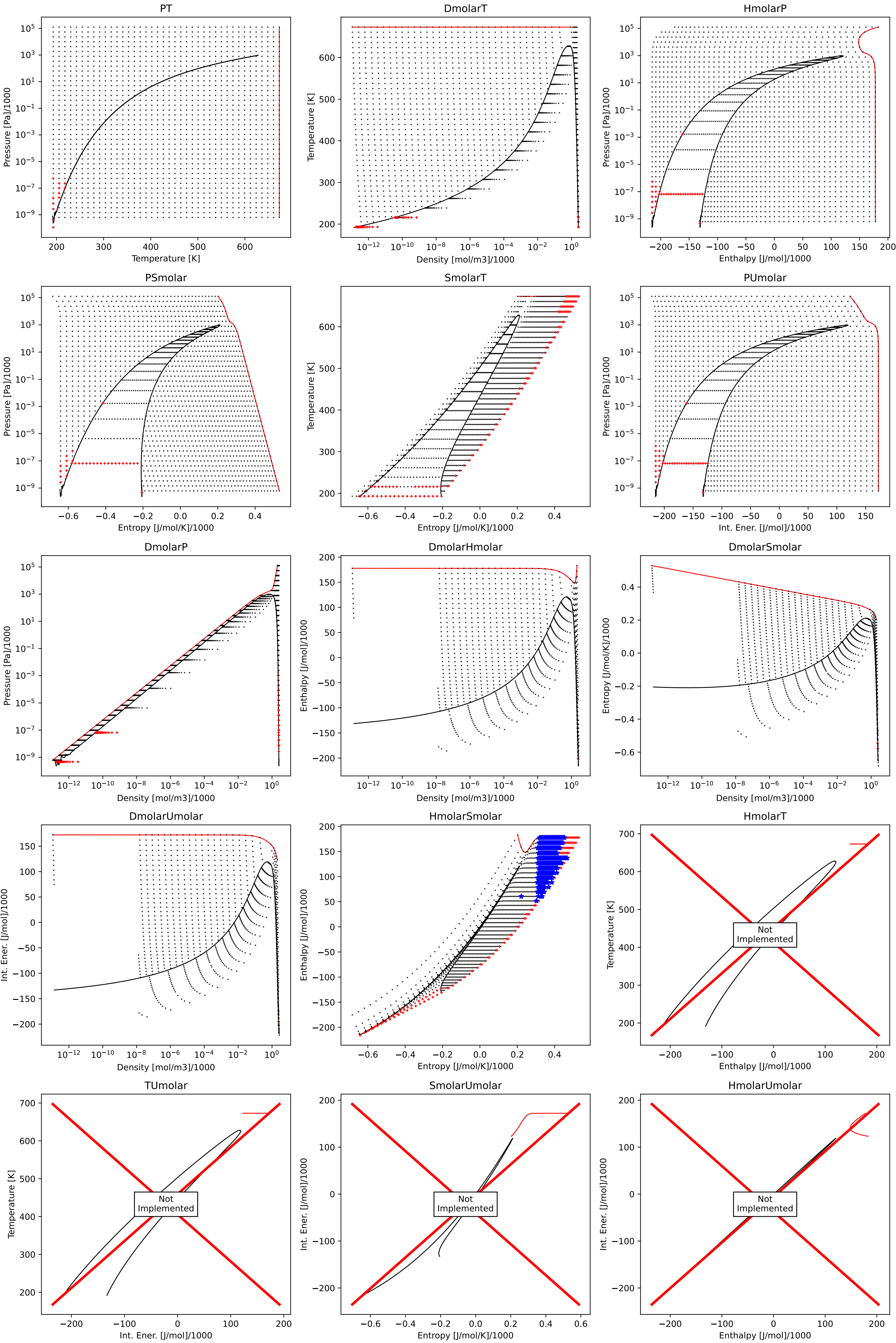
Consistency plots for MD3M
