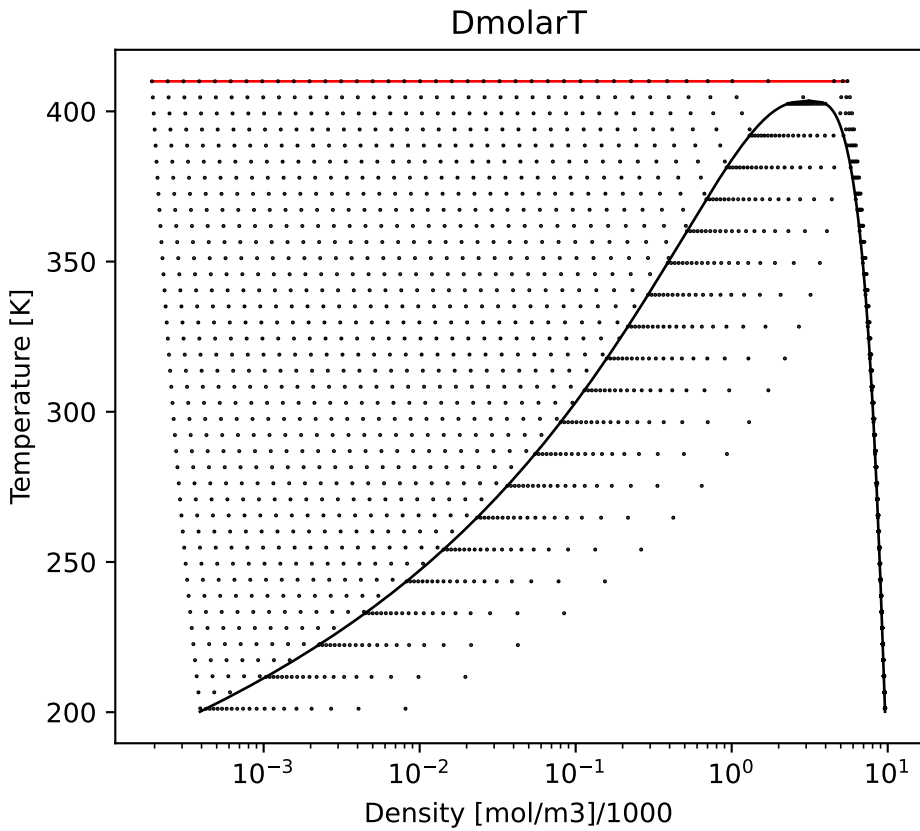
Consistency plots for R1336MZZE
