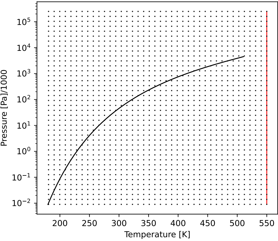
PSmolar
