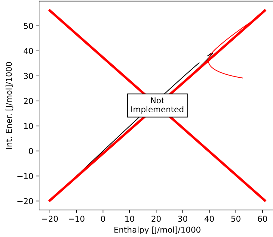
HmolarUmolar
