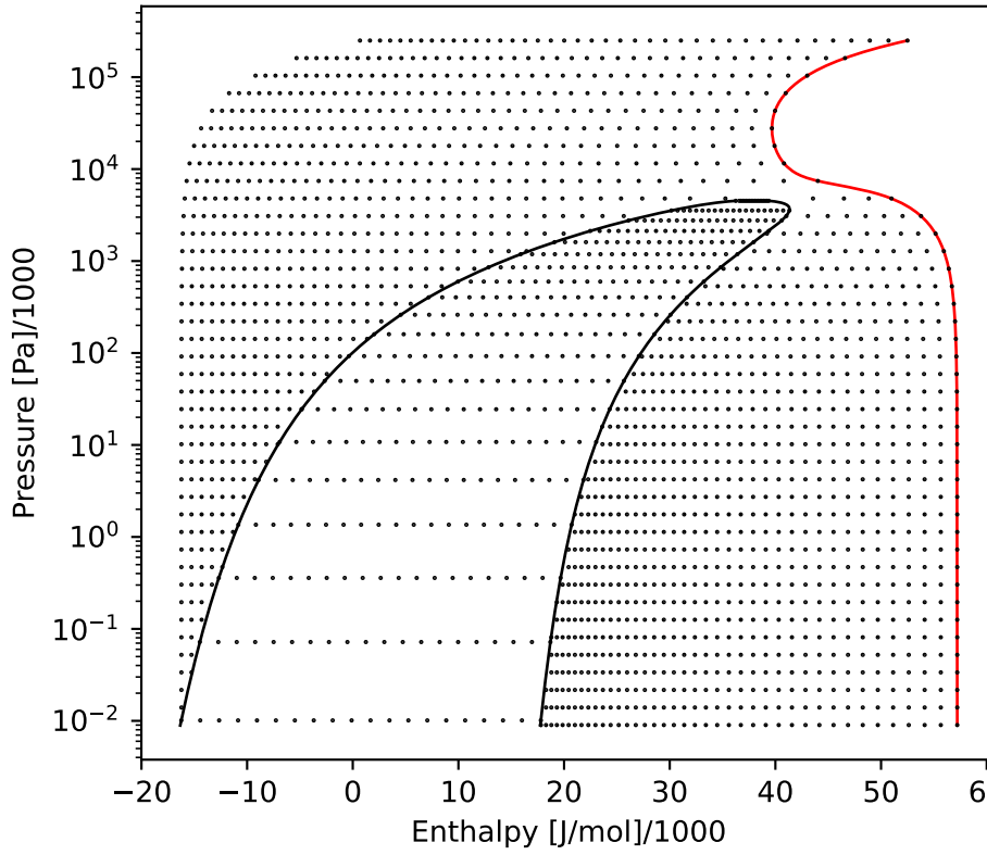
PUmolar
