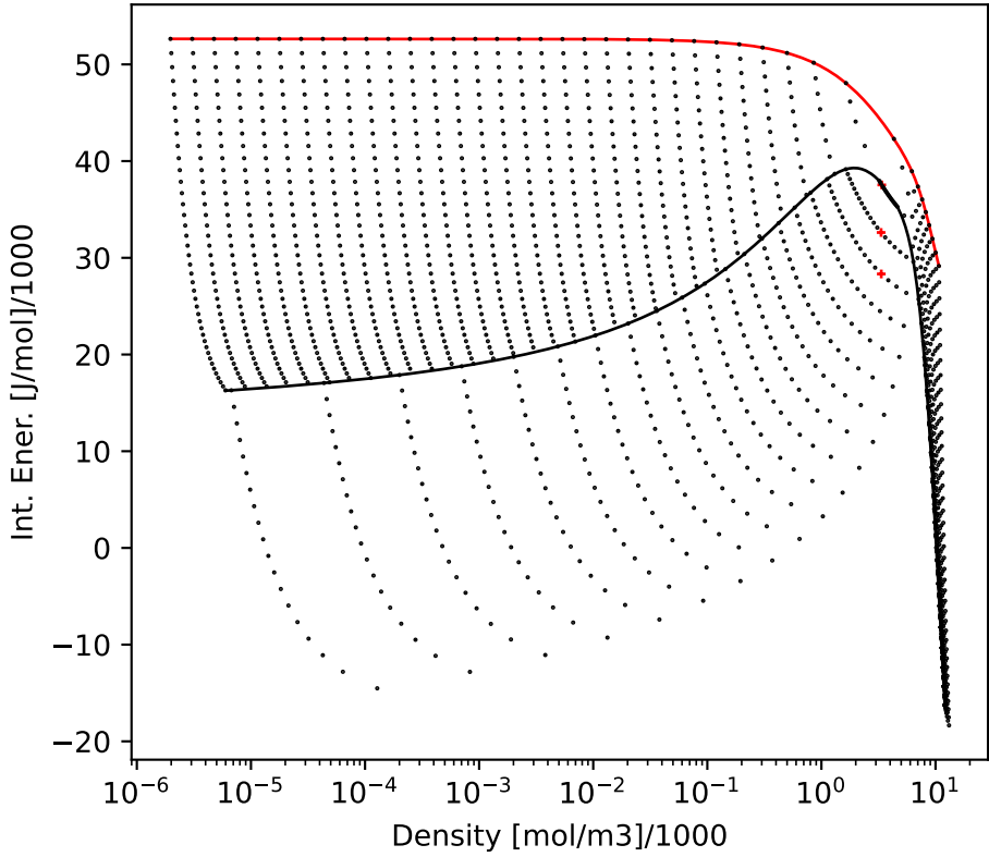
TUmolar
