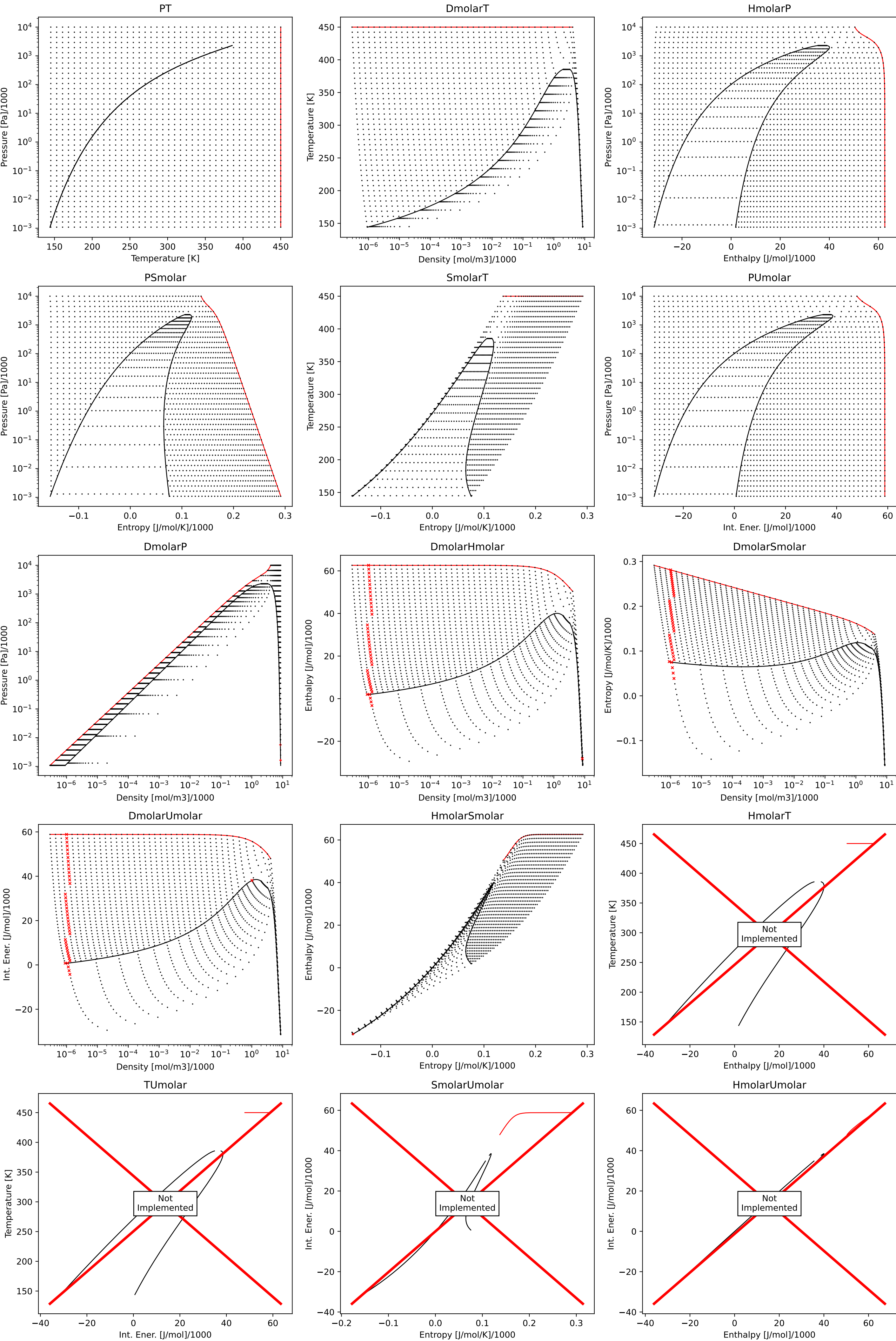
Consistency plots for n-Perfluorobutane
