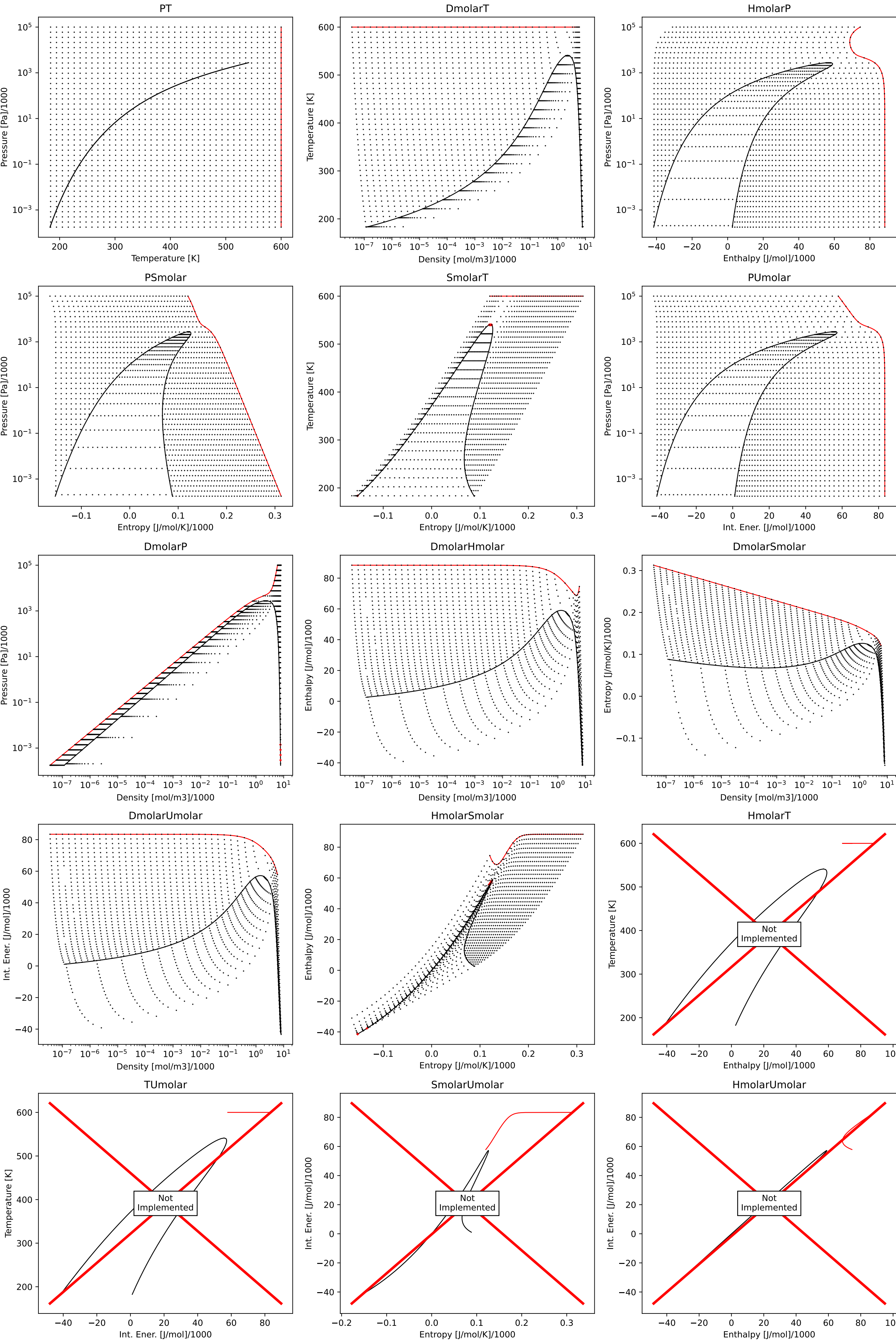
Consistency plots for n-Heptane
