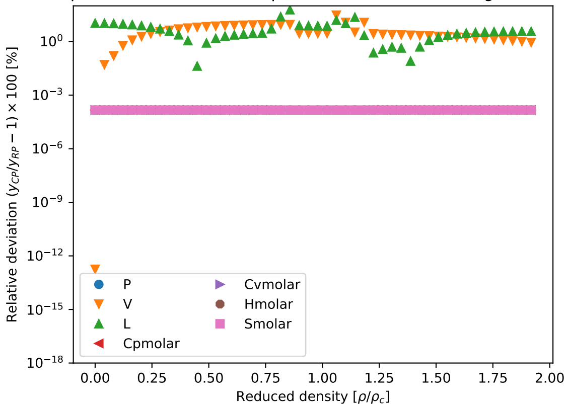
Comparison between CoolProp and REFPROP(10.0) along T = 1.01 \cdot T_c
