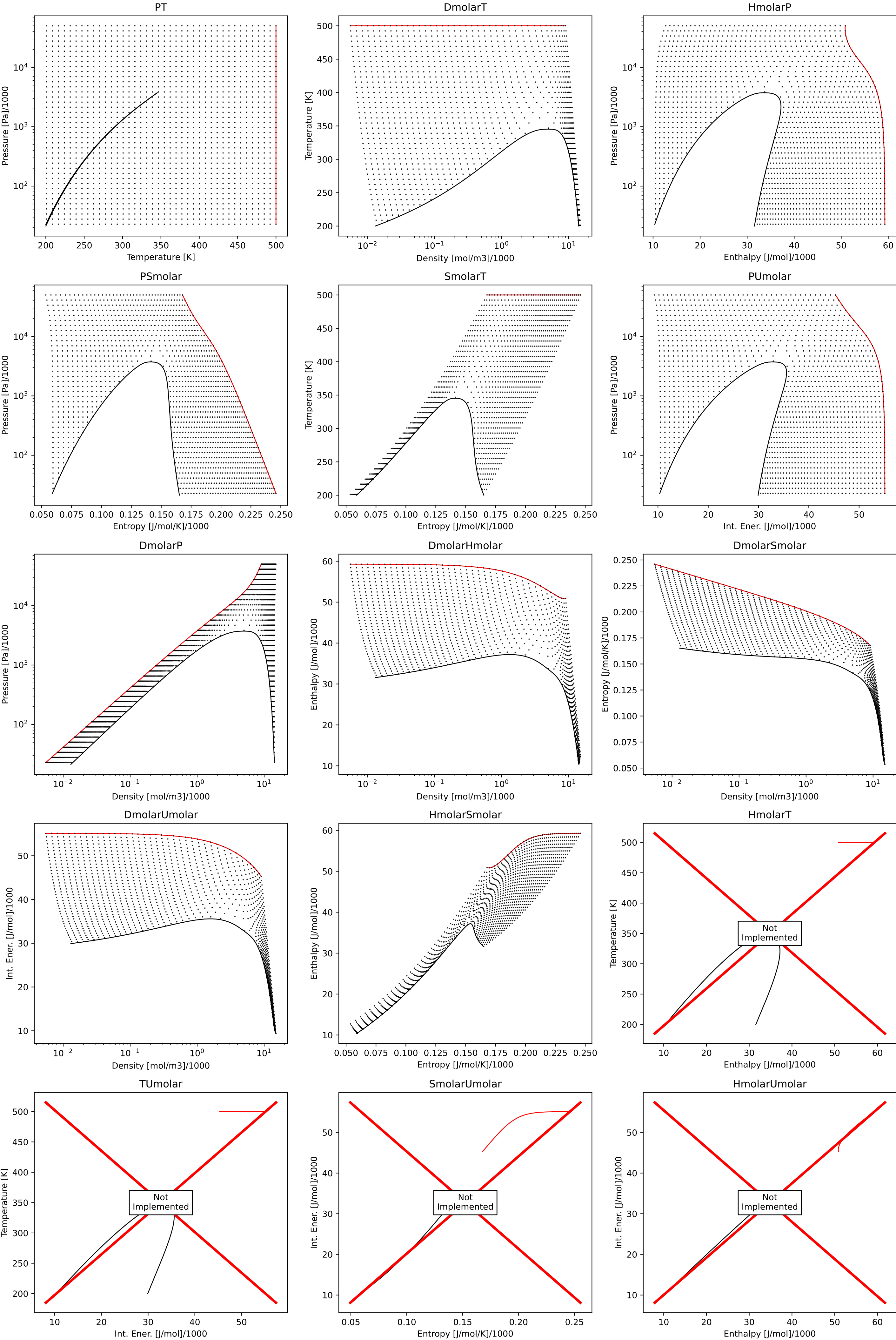
Consistency plots for R404A
