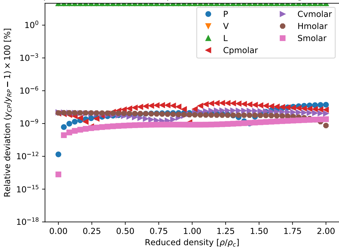
Comparison between CoolProp and REFPROP(10.0) along T = 1.01 \cdot T_c
