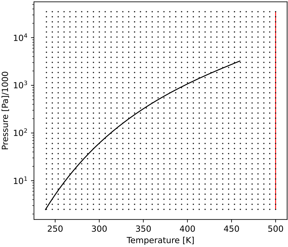
PSmolar
