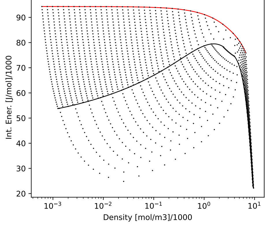
TUmolar
