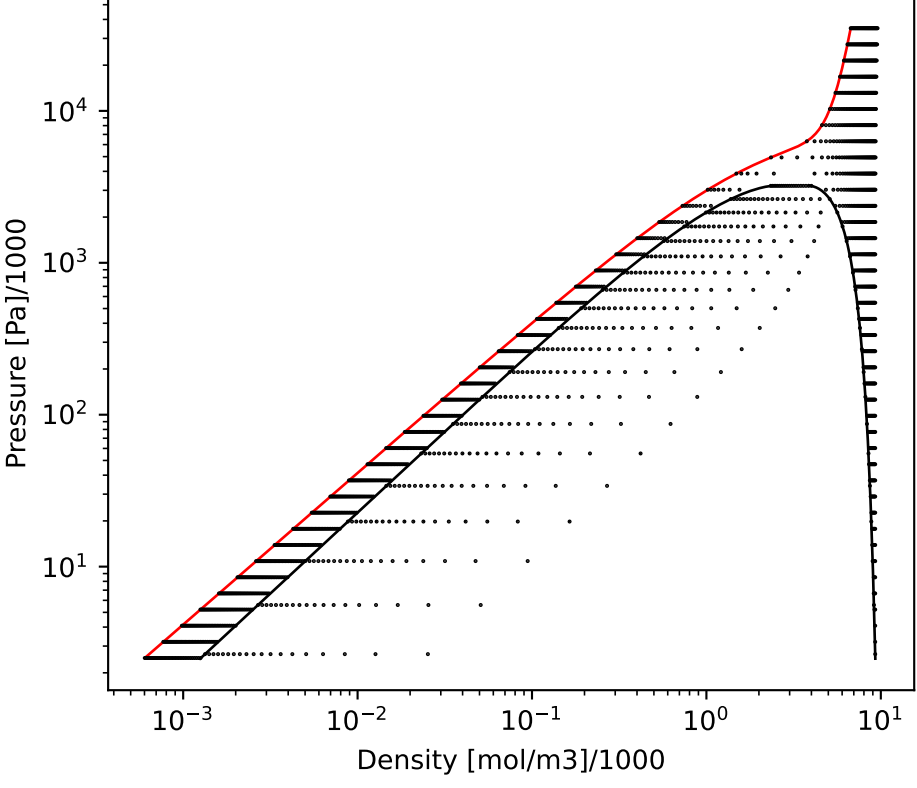
DmolarUmolar
