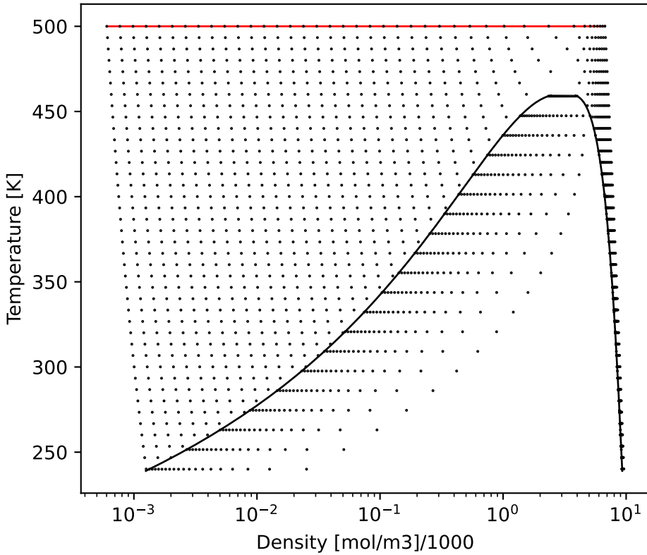
SmolarT
