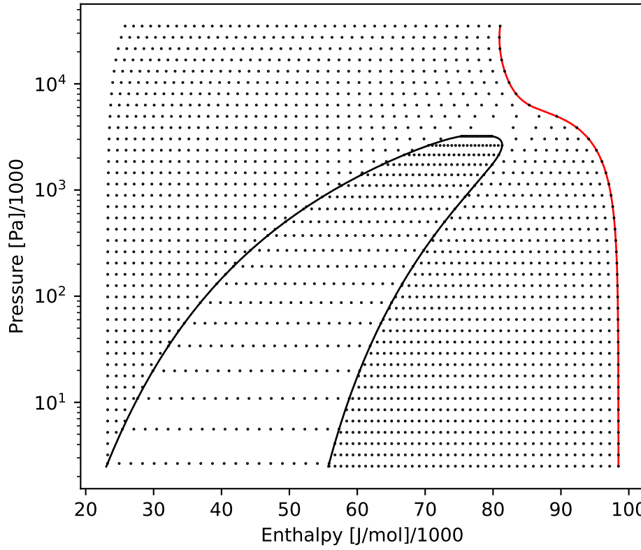
PUmolar
