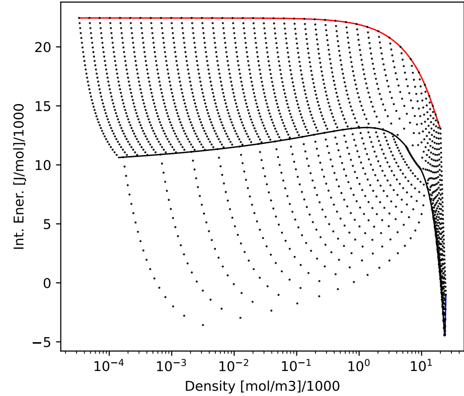
TUmolar
