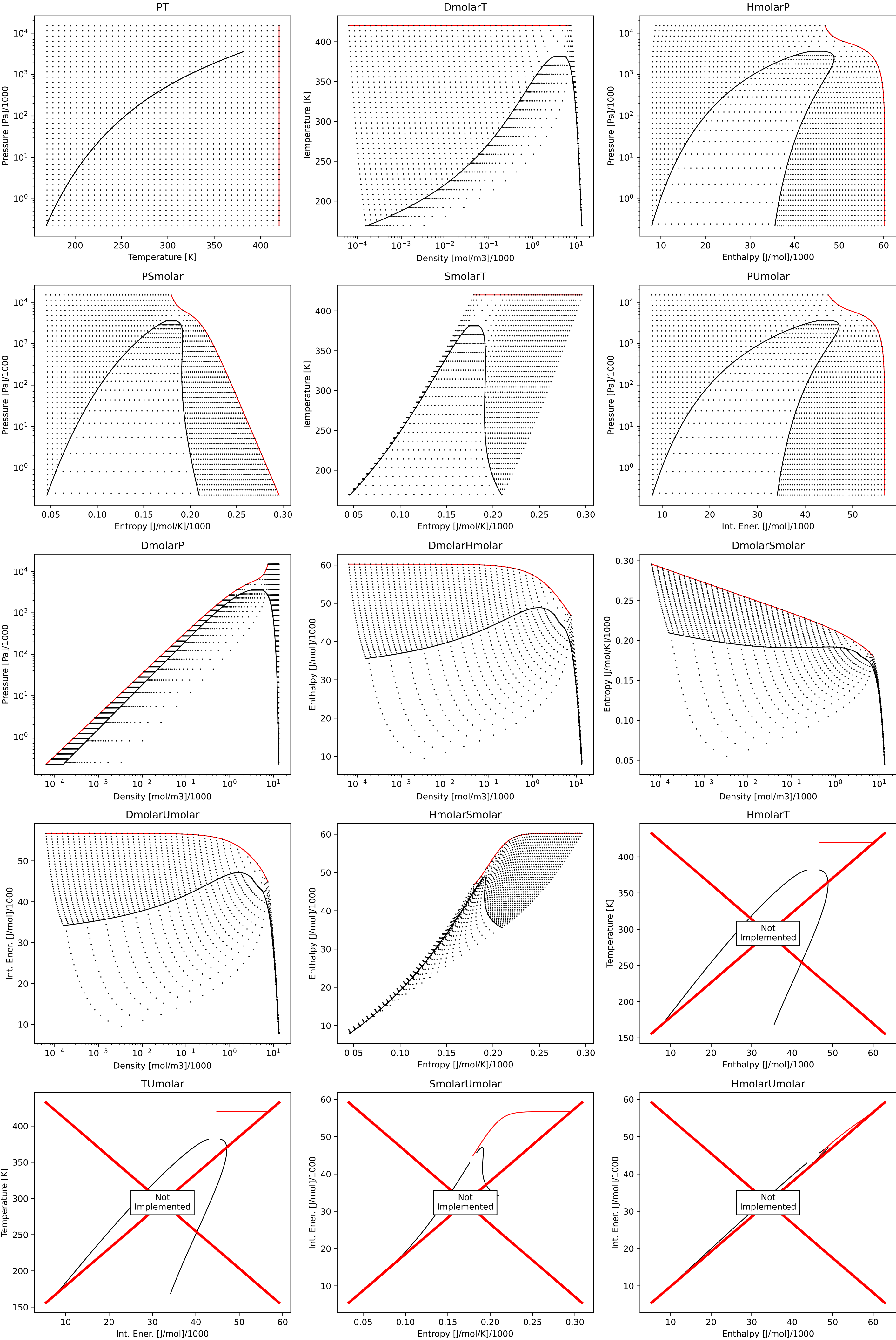
Consistency plots for R1234ze(E)
