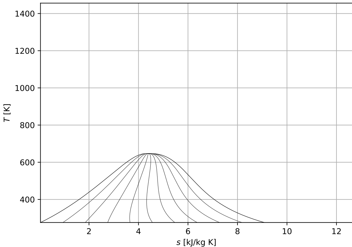
T, s Graph for Water
