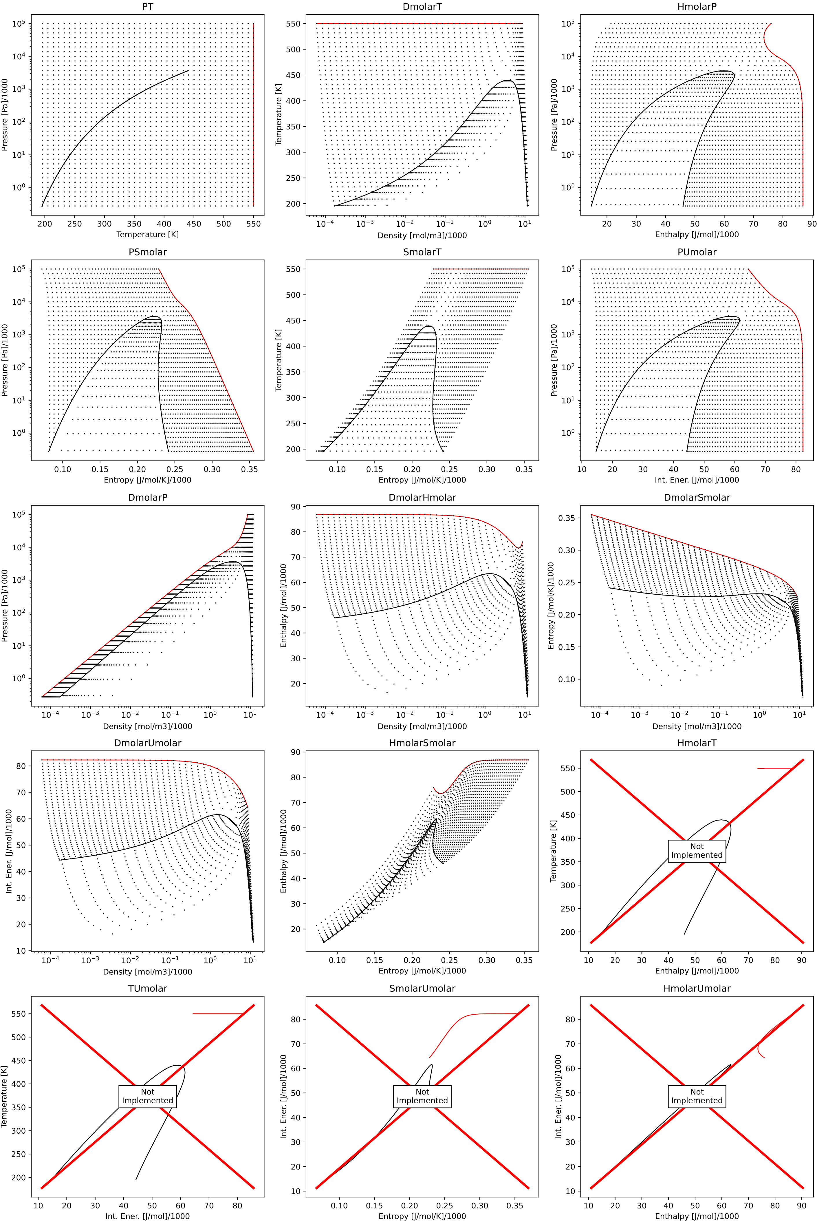
Consistency plots for R1233zd(E)
