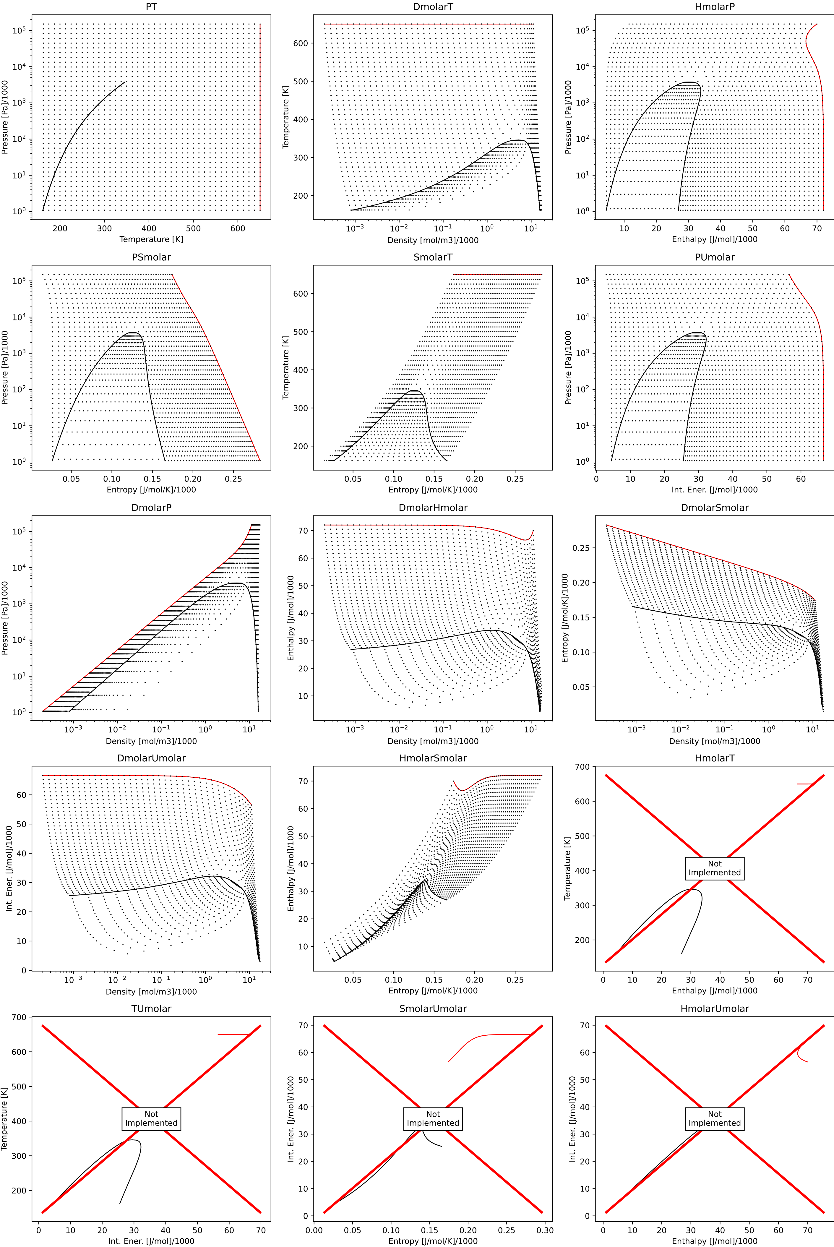
Consistency plots for R143a
