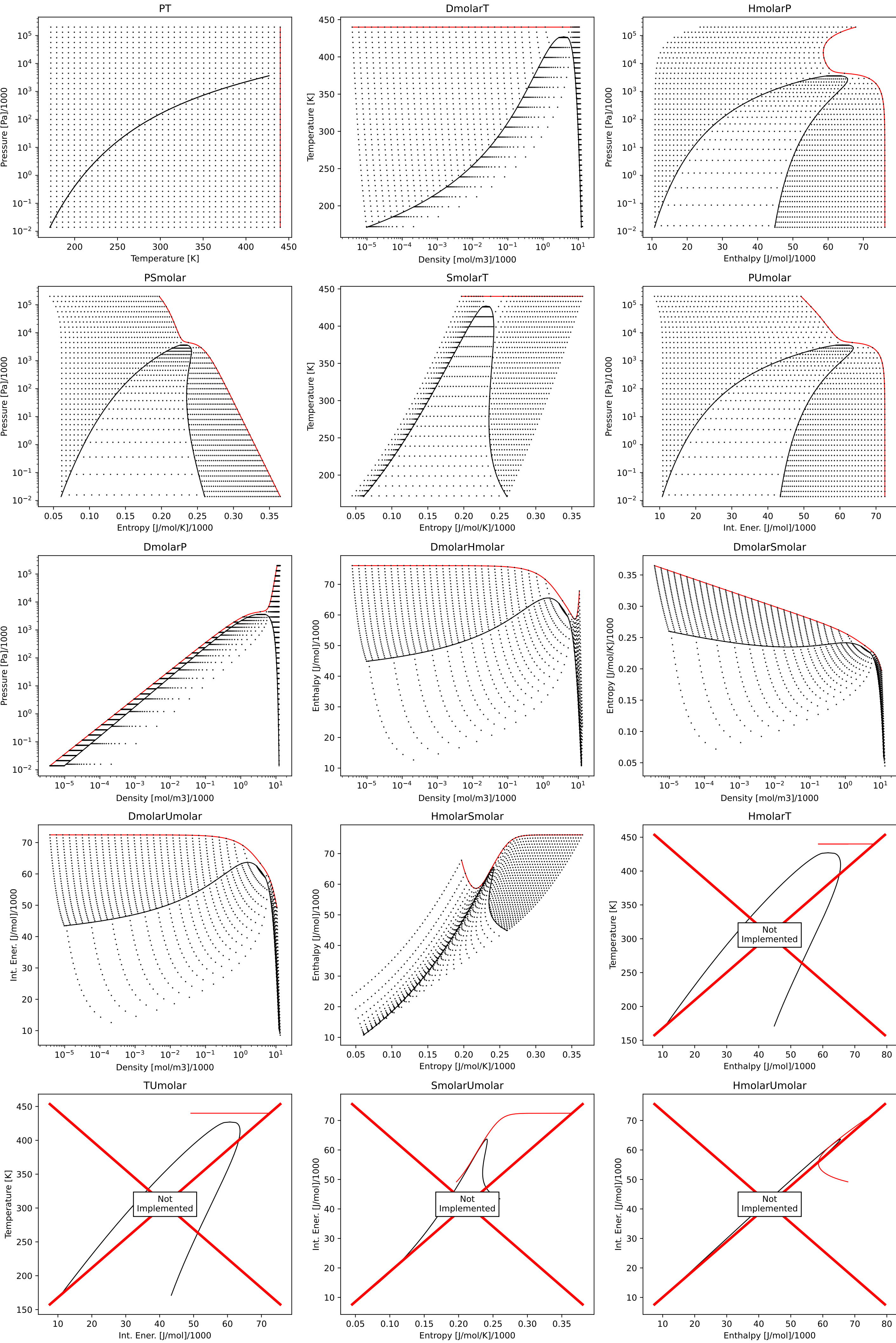
Consistency plots for R245fa
